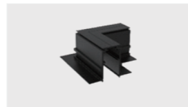
L-shaped (Downward) Art.127.44.40 Material: AL6063-T5 Size: L95×W95×H46.5mm
